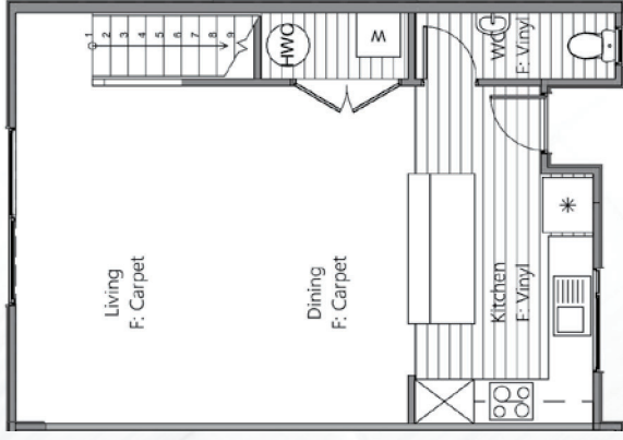
LOT 2 | Ground Floor
